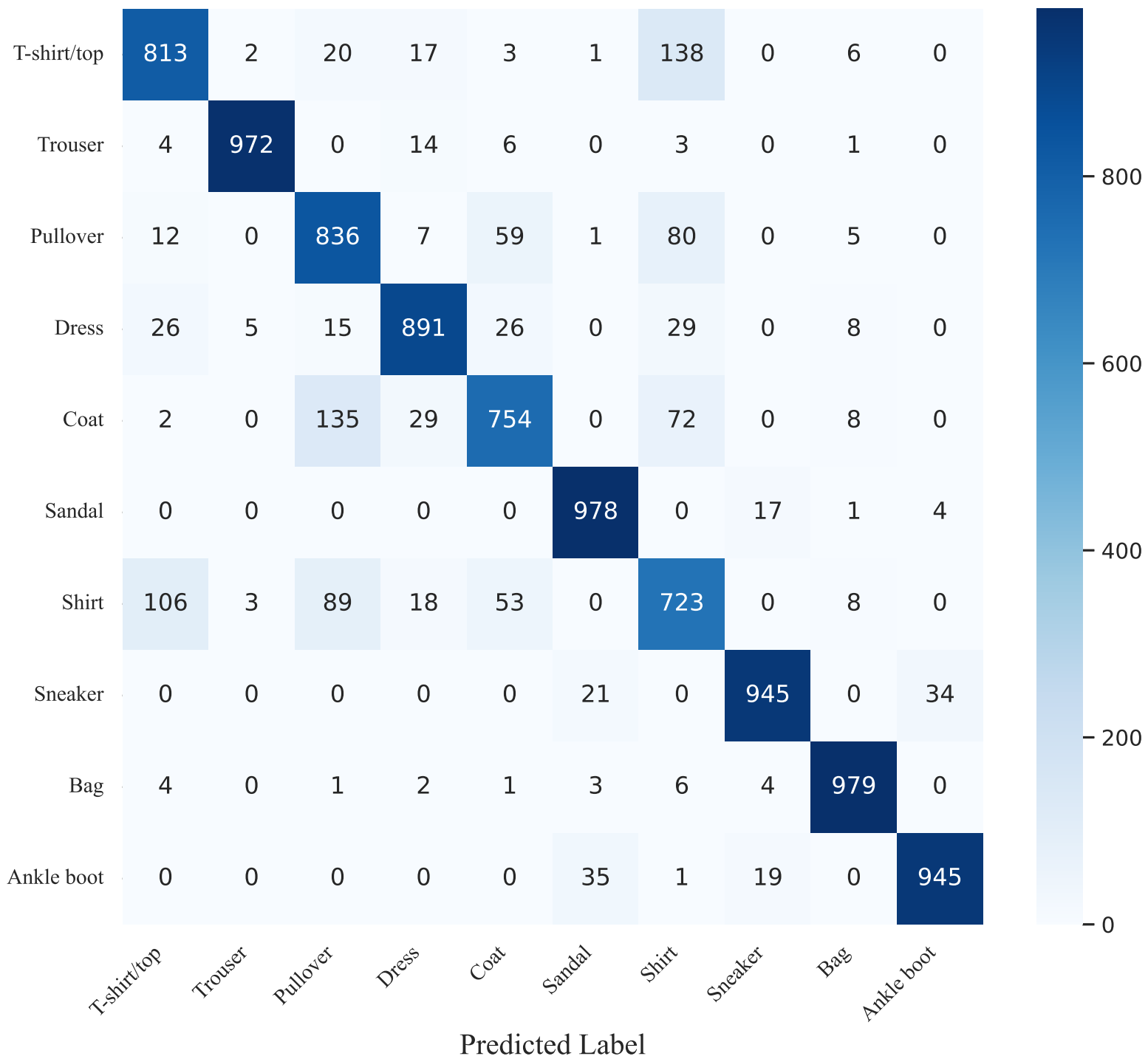
Confusion Matrix -- Baseline Model
